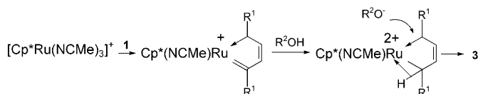
Scheme 2. Proposed mechanism for the formation of dienyl ethers 3 .
